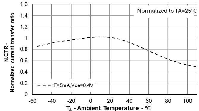
Figure 12. Normalized Current Transfer Ratio vs. Forward Current vs. Ambient Temperature(Vce=0.4V)
